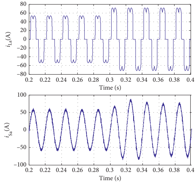
FIGURE 19: Waveforms of load current and source current in the case of abrupt loading.
