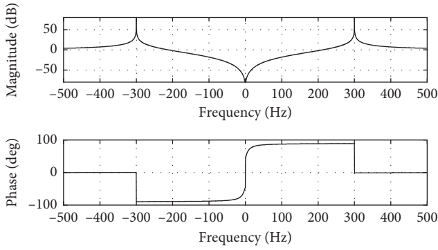
FIGURE 2: Bode diagram of VR controller.
