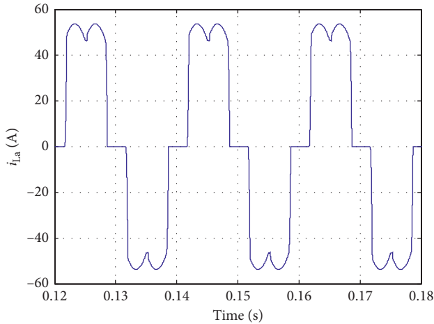
FIGURE 10: Waveform of nonlinear load current.
