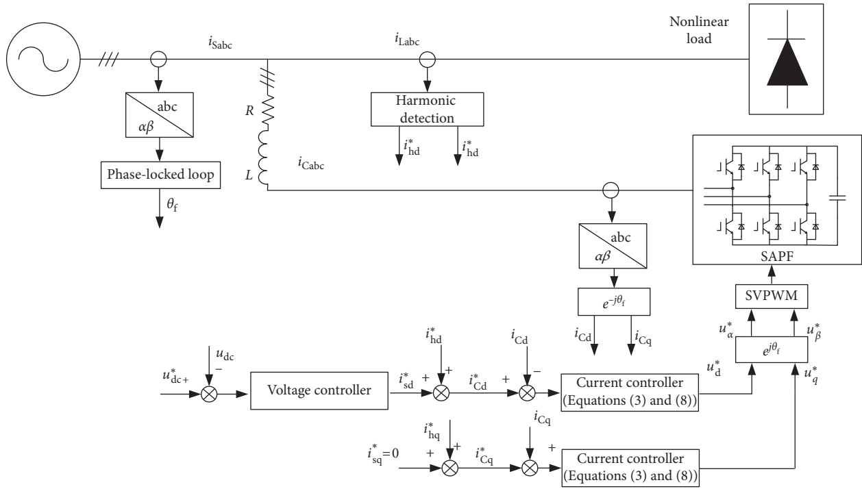
FIGURE 9: Control block diagram of three-phase three-wire SAPF.
