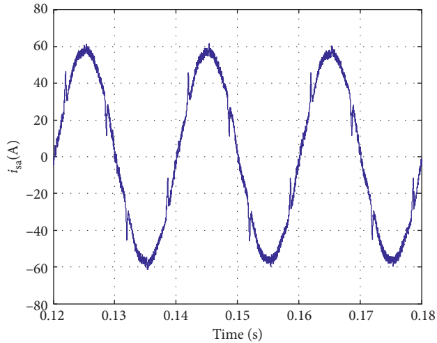
FIGURE 15: Waveform of source current using PI controller and 6th VR controller.
