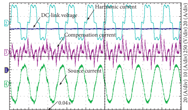
FIGURE 23: Experimental dynamic waveform after adding VR controller.
