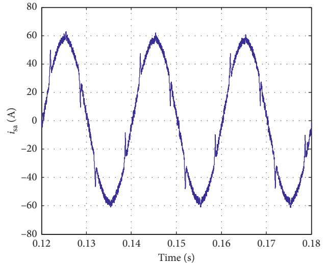
FIGURE 13: Waveform of source current using PI controller.
