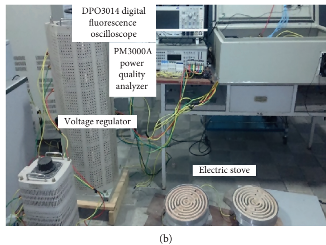
FIGURE 20: Experimental setups of SAPF.
