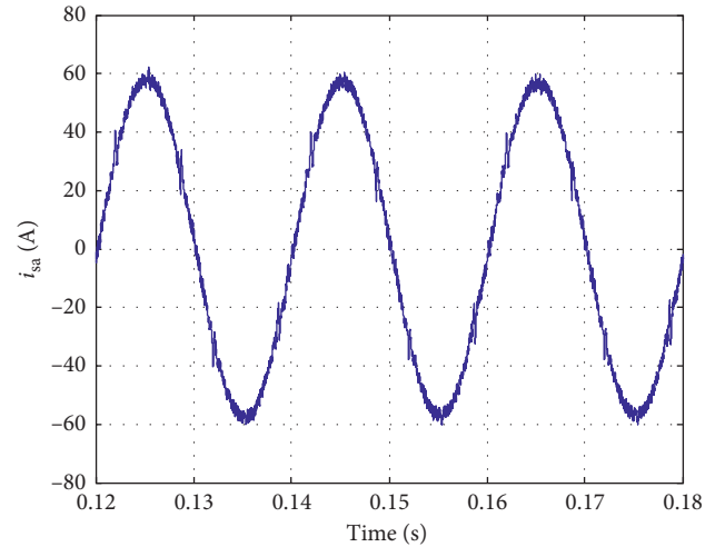
FIGURE 17: Waveform of source current using PI controller and multi-VR controllers.
