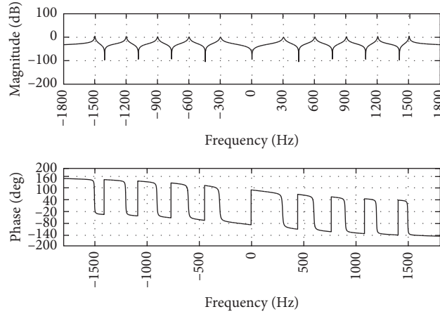
FIGURE 8: Bode diagram of closed loop current considering digital control delay.
