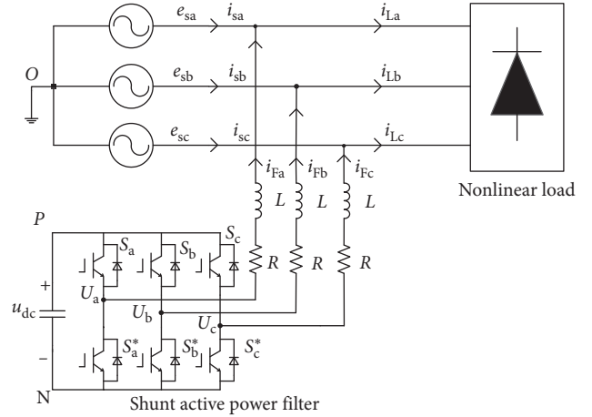
FIGURE 1: Structure of three-phase three-wire SAPF.
