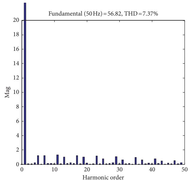
FIGURE 14: FFT analysis of source current using PI controller.
