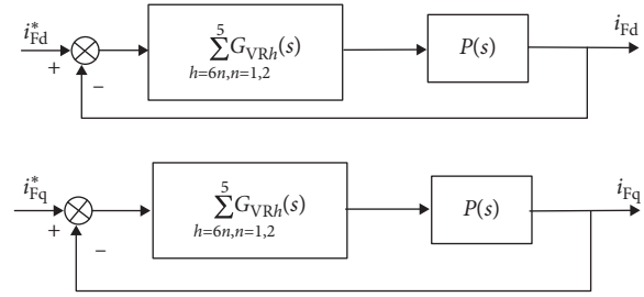
FIGURE 3: Current control block diagram based on multi-VR controller.
