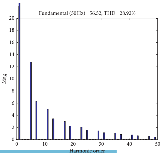
FIGURE 12: FFT analysis of nonlinear load current.
