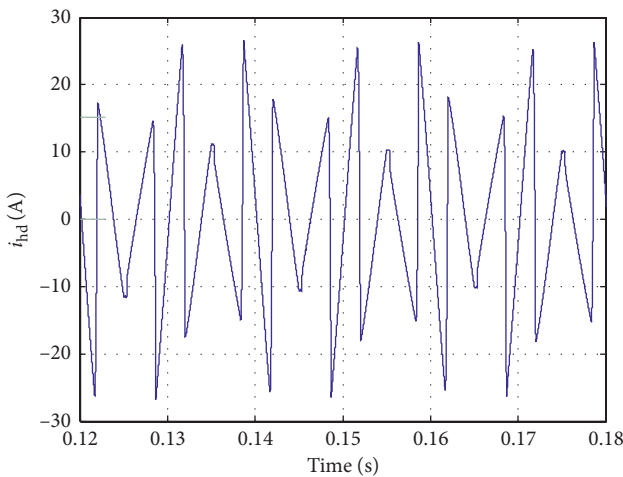
FIGURE 11: Waveform of harmonic currents.
