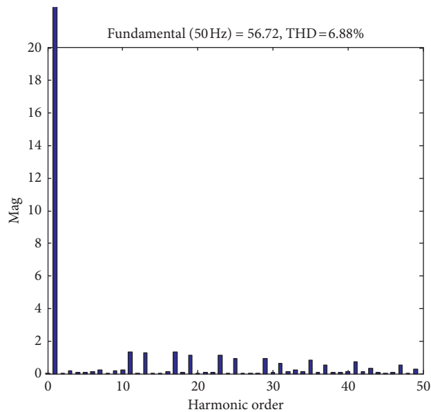
FIGURE 16: FFT analysis of nonlinear load current using PI controller and 6th VR controller.
