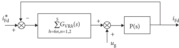
FIGURE 5: Current control block diagram when the system is disturbed by the grid voltage.
