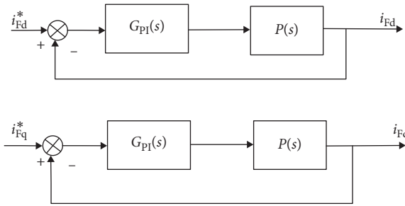
FIGURE 6: Fundamental current control block diagram based on PI controller.
