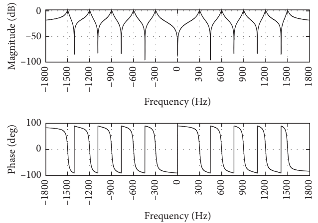
FIGURE 4: Bode diagram of harmonic current close loop control.
