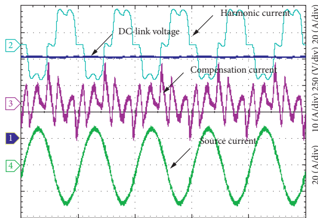
FIGURE 22: Experimental steady waves for proposed scheme.
