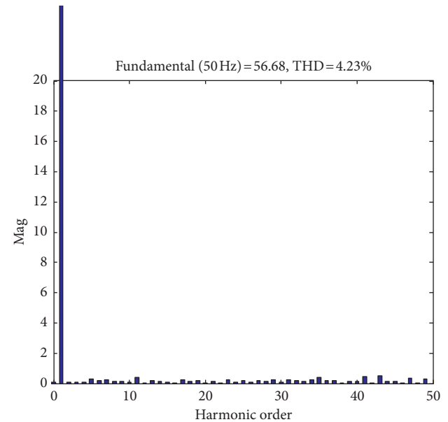
FIGURE 18: FFT analysis of nonlinear load current using PI controller and multi-VR controllers.
