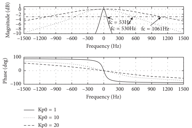
FIGURE 7: Bode diagram of fundamental close loop control.
