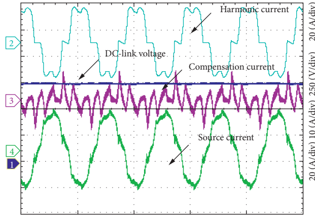
FIGURE 21: Experimental steady waves using PI controller.
